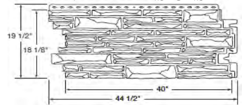
PANEL DIMENSIONS
